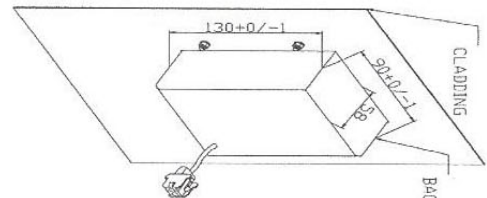
ASSEMBLED BACK VIEW SCALE 1:2
